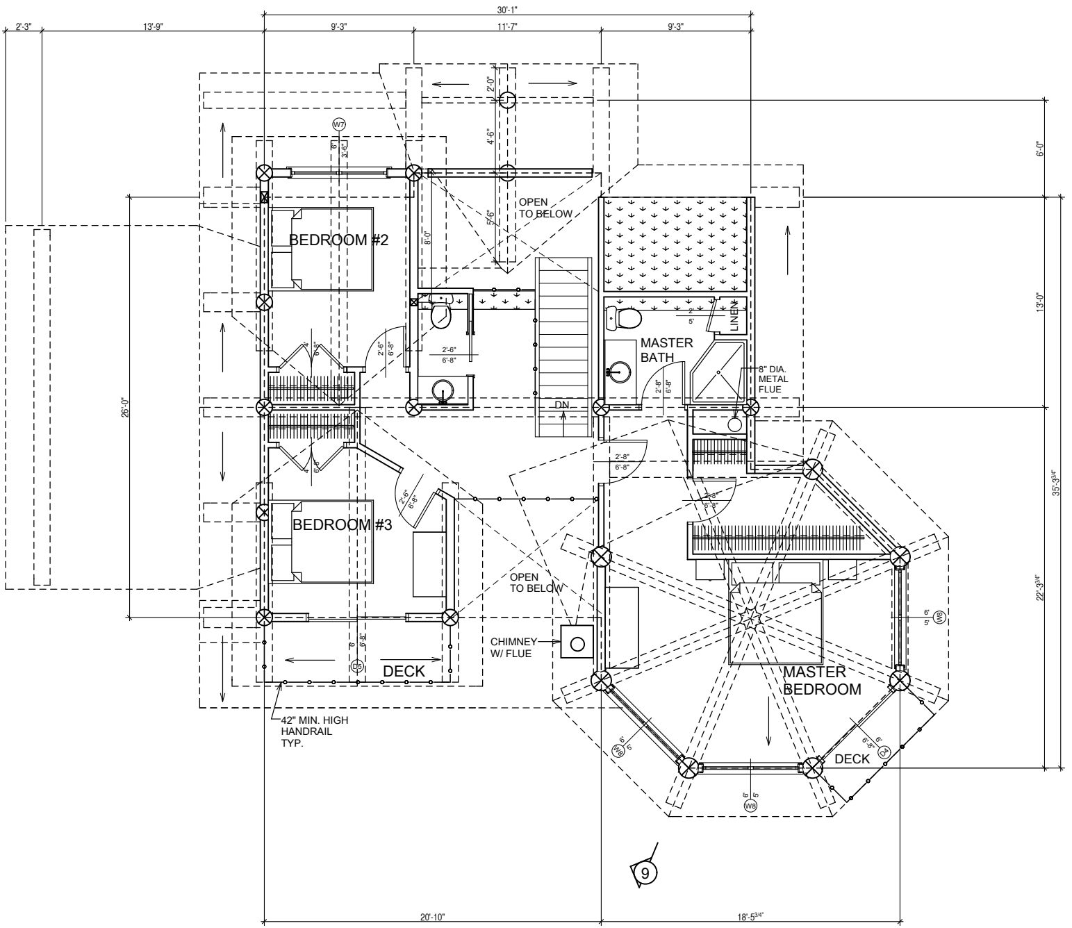
SECOND FLOOR PLAN AREA: 760 SQ. FT. SNOW LOAD: 69 PSF
